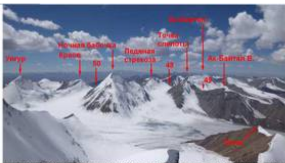
Panorama from Rock Horse looking west. (L to R) Ughur (4979m), Peak Kralow (4941m), Nochnoi Motyl (Night Butterfly, 5065m), Lednaya Str'el'ca (4892m), Akbatal-Pt Blindness (4970m), Akbatal (4981m) and Akbatal Vostok (4743m). Kucyk (Pony, 4705m) is visible in the lower right foreground (V. Zholsberka)
